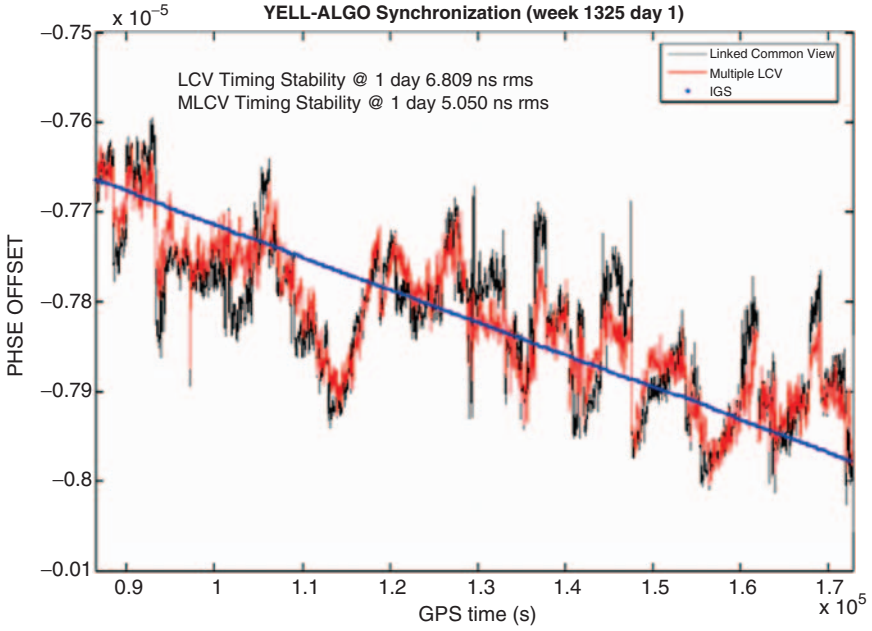
Fig. 11. YELL-ALGO synchronization.
